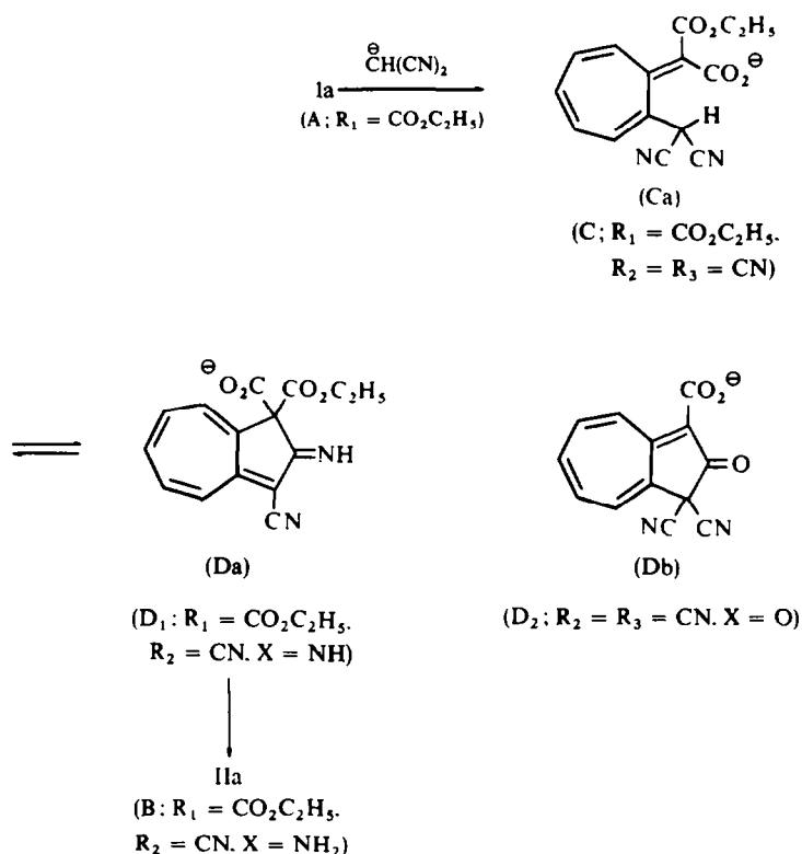
CHART 2. The reaction of 3-ethoxycarbonyl-2H-cyclohepta[b]furan-2-one (Ia) and malononitrile
